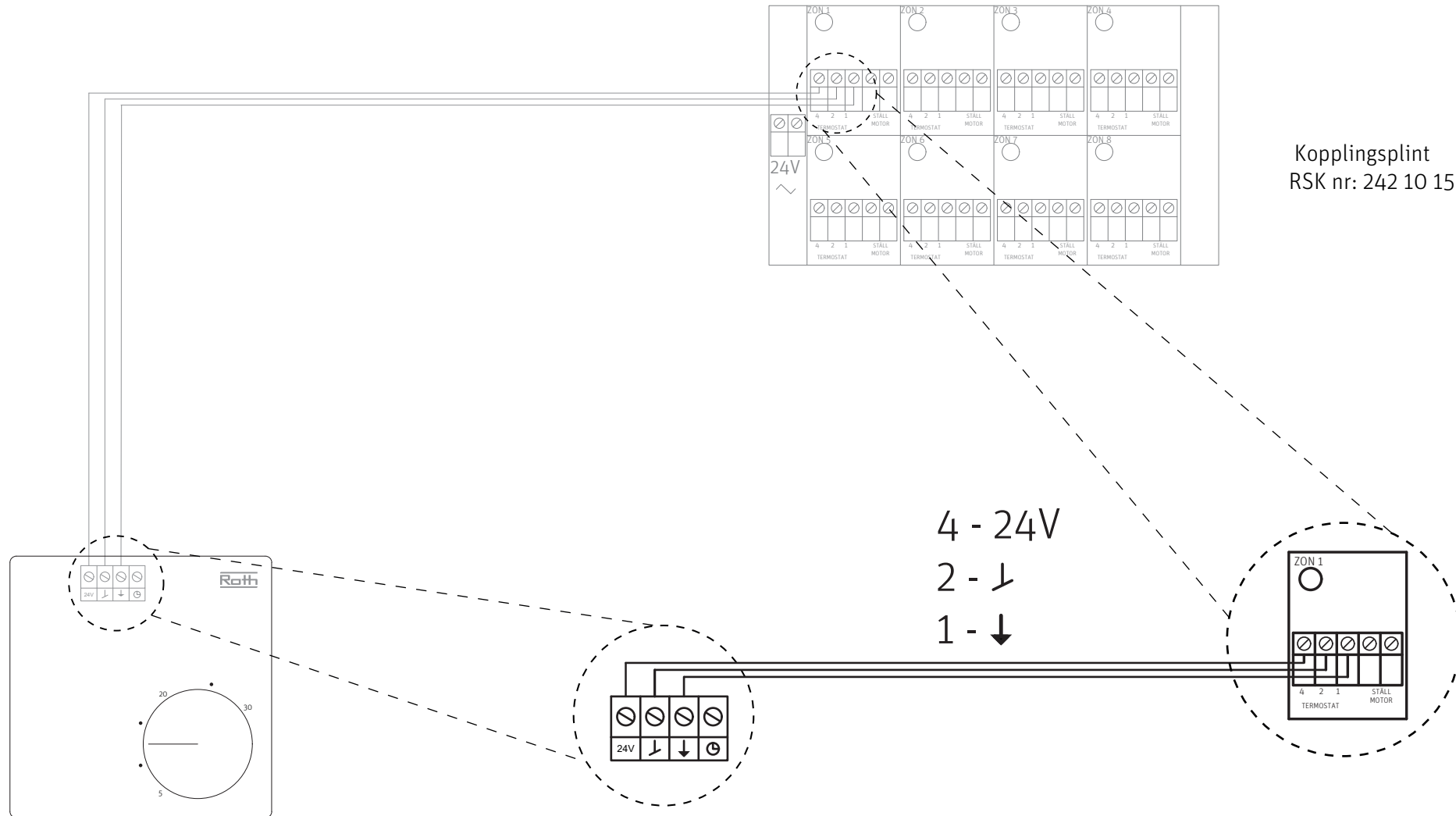
Roth Touchline® BL rumstermostat RSK nr: 242 63 87
