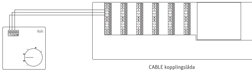
Roth Touchline® BL rumstermostat RSK nr: 242 63 87
